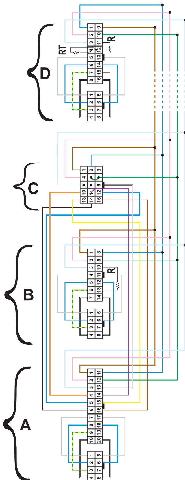
fig. 125- Module connection cable wiring diagram
