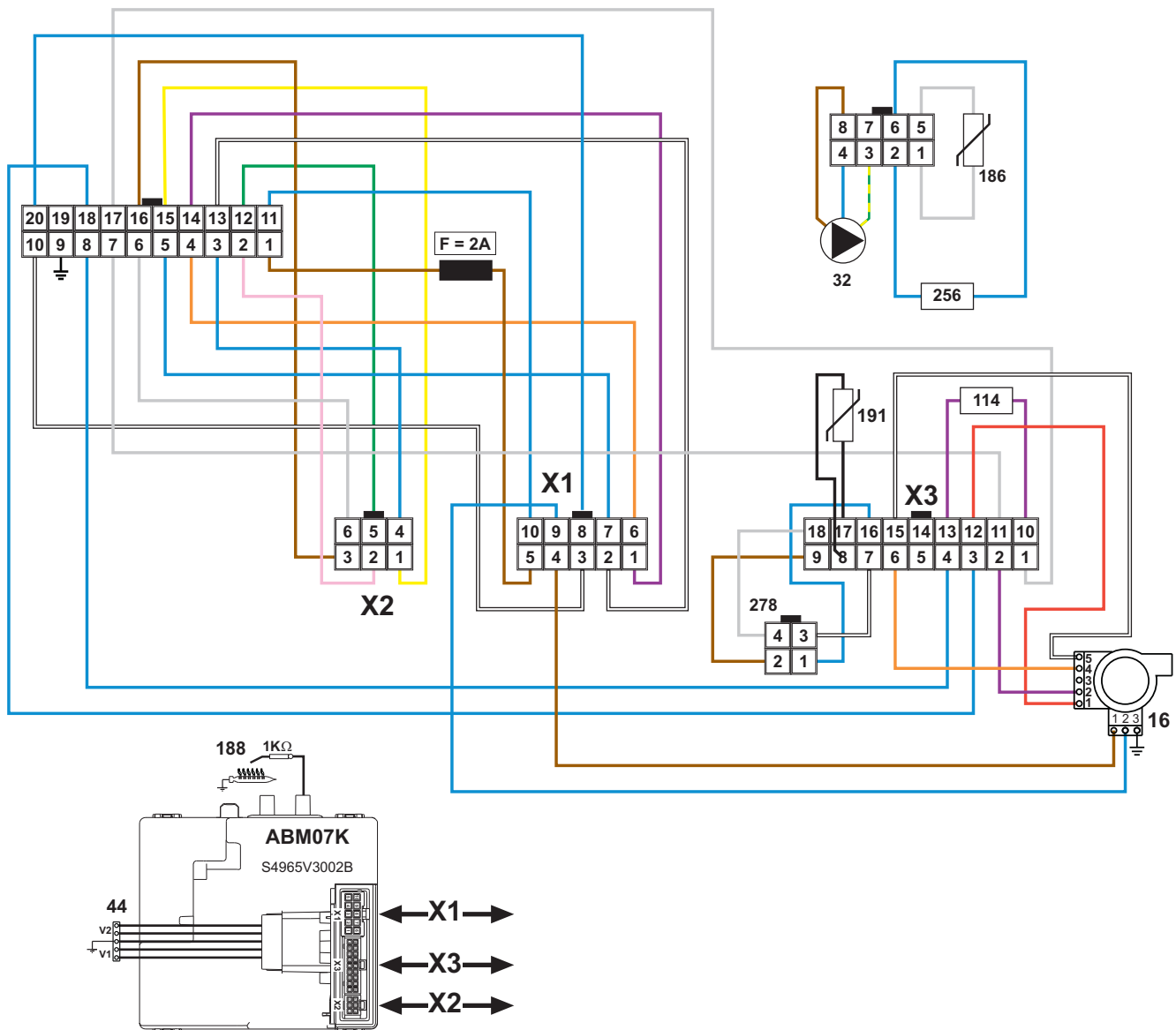
fig. 122- First module wiring diagram
