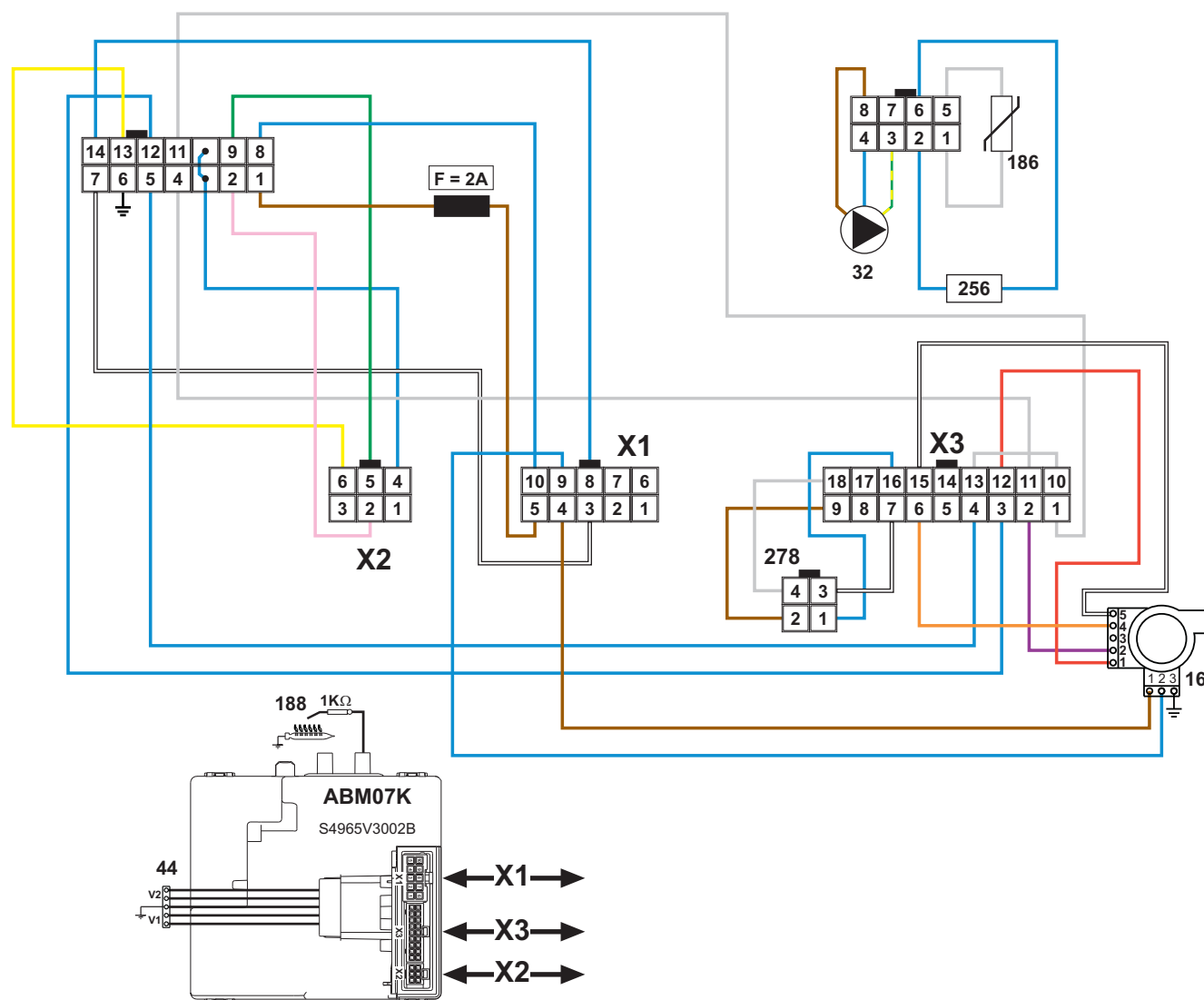
fig. 123- Intermediate module wiring diagram
