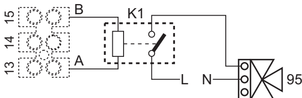
fig. 118- Connection of the 3-way valve with 2 wires
