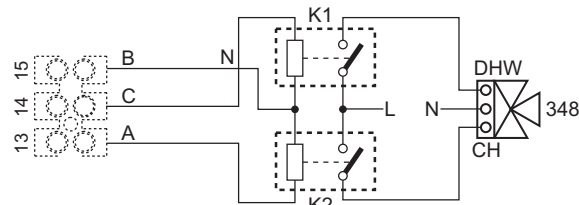
fig. 119- Connection of the 3-way valve with 3 wires
